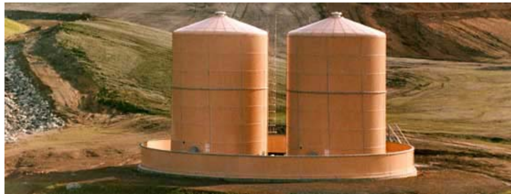
Steel Knuckle Roof Tanks with Secondary Containment Ring
