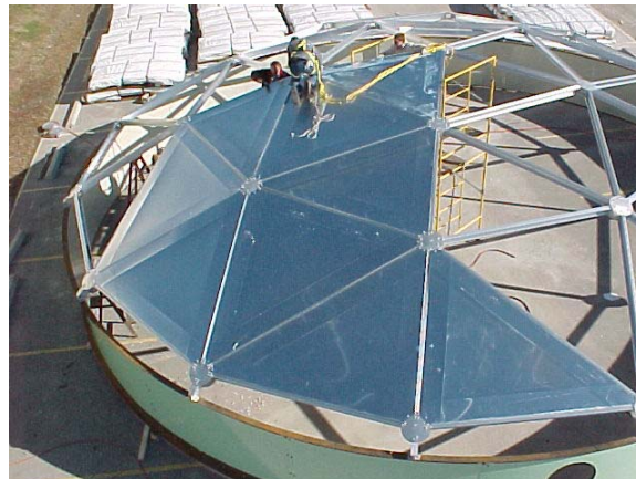
Geodesic Dome Assembly
